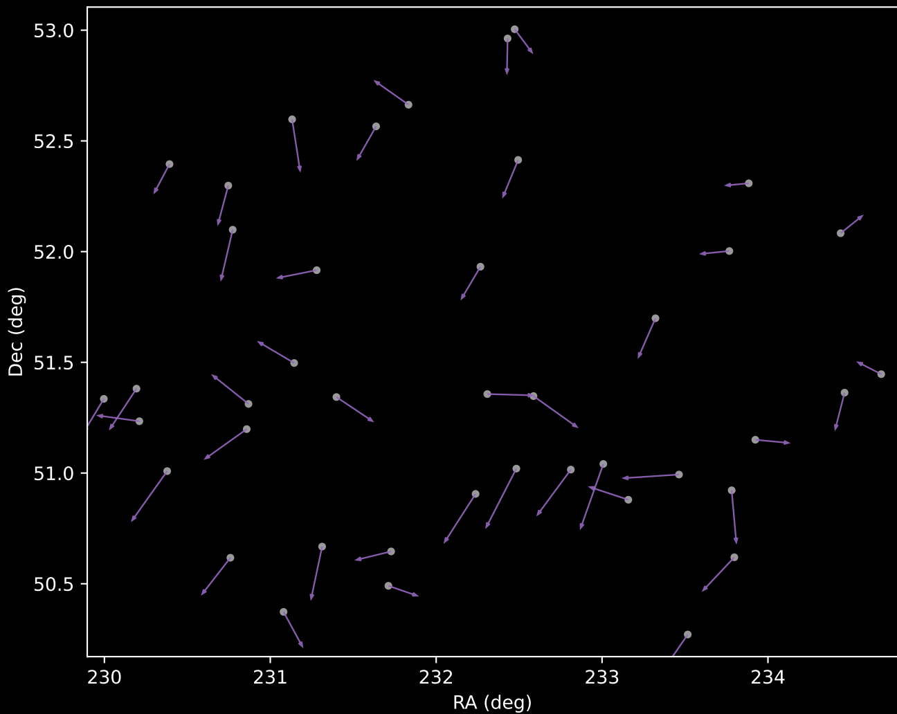
APOGEE DR17 Cluster 8 Proper Motion Vectors (n=42)
