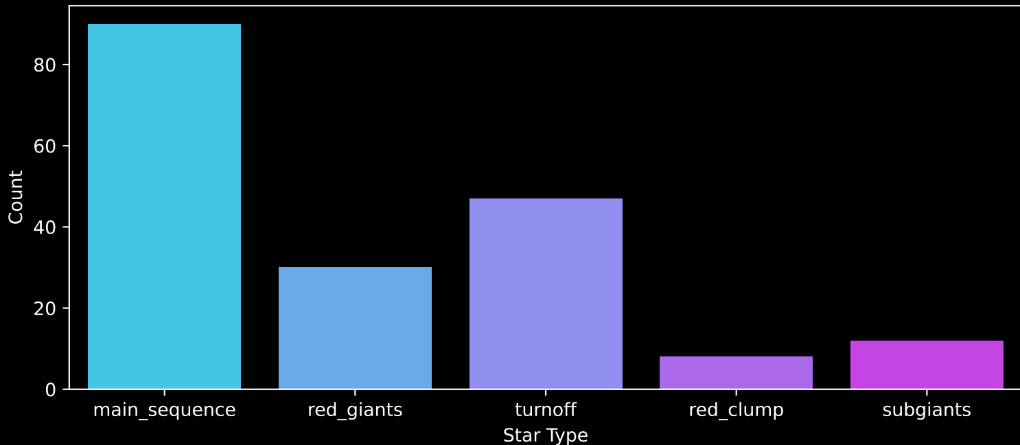
APOGEE DR17 Field: [167+39_MGA] Count plot of Star Type
