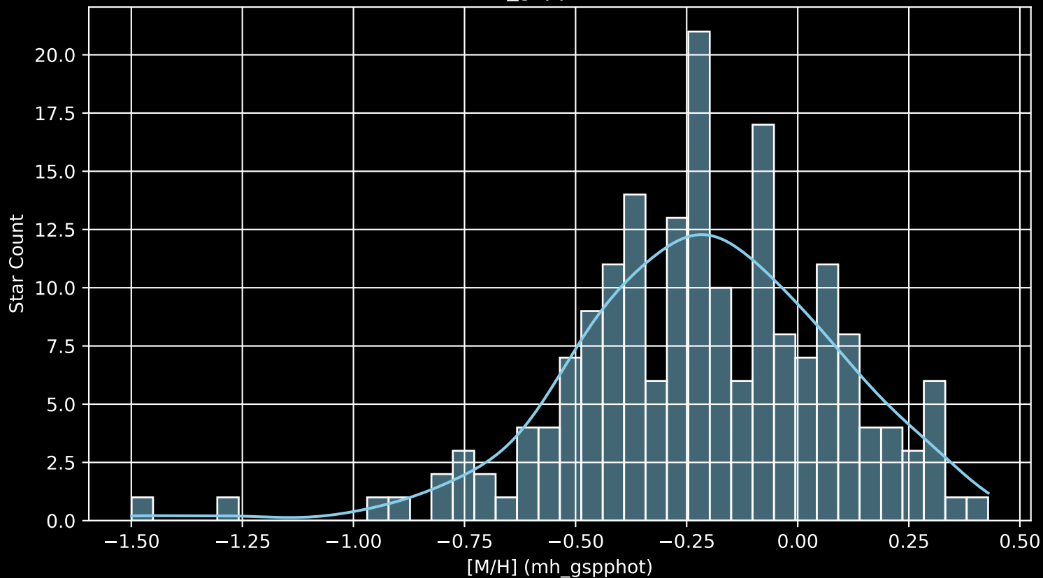
APOGEE DR17 Field: [167+39_MGA [M/H] (mh_gspphot) (n= 187)
