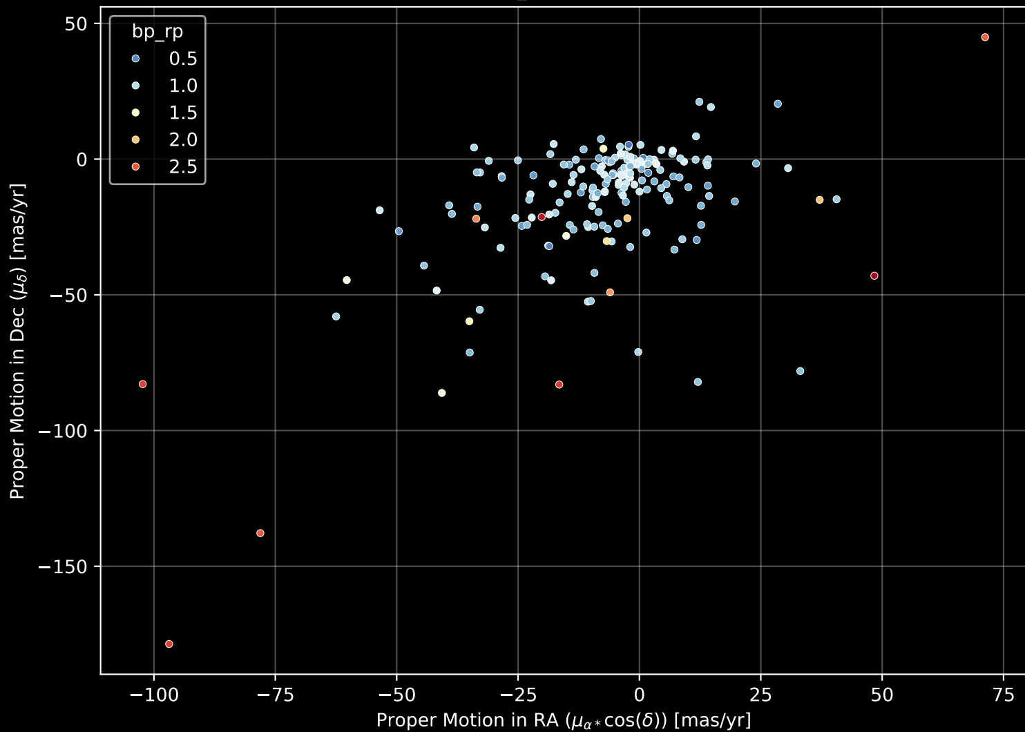
APOGEE DR17 Field: [167+39_MGA] Proper Motion Diagram (n= 187)
