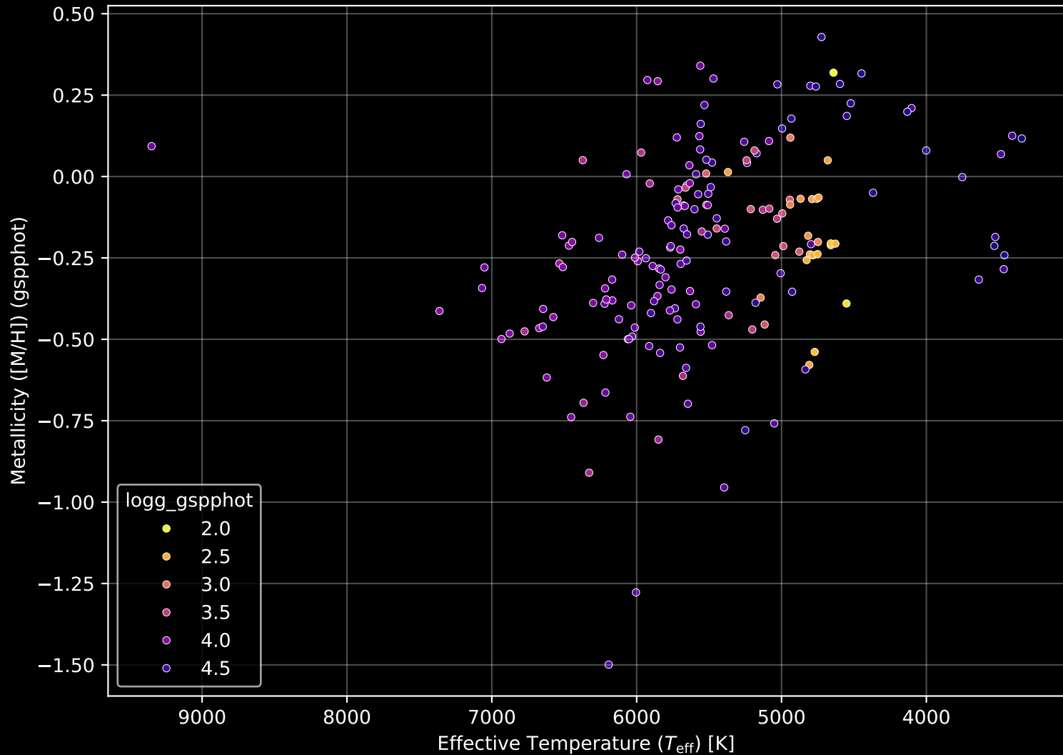
APOGEE DR17 Field: [167+39_MGA] Stellar Population Parameters (n= 187)
