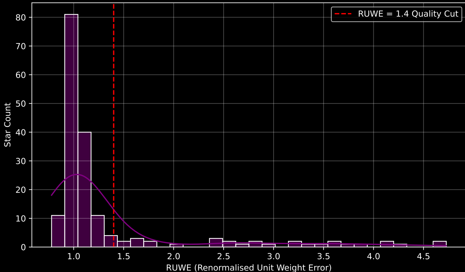
GAPOGEE DR17 Field [167+39_MGA] RUWE Distribution (n= 177)
