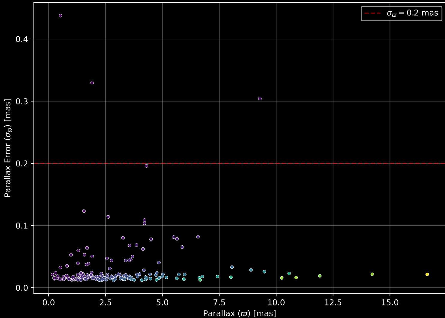
APOGEE DR17 Field: [167+39_MGA] Parallax Quality (n= 187)
