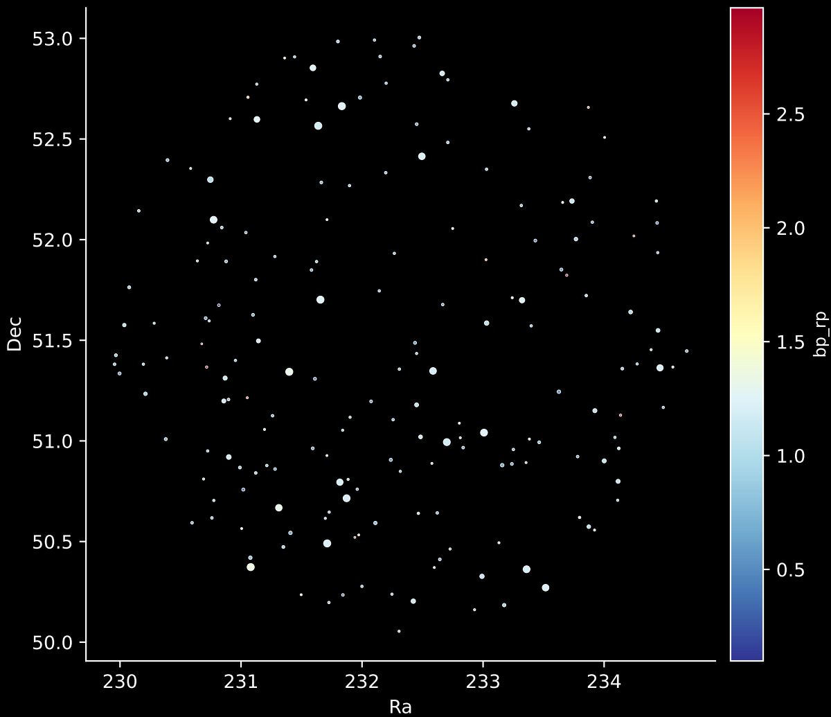
APOGEE DR17 Field: [167+39_MGA] Stars: 187
